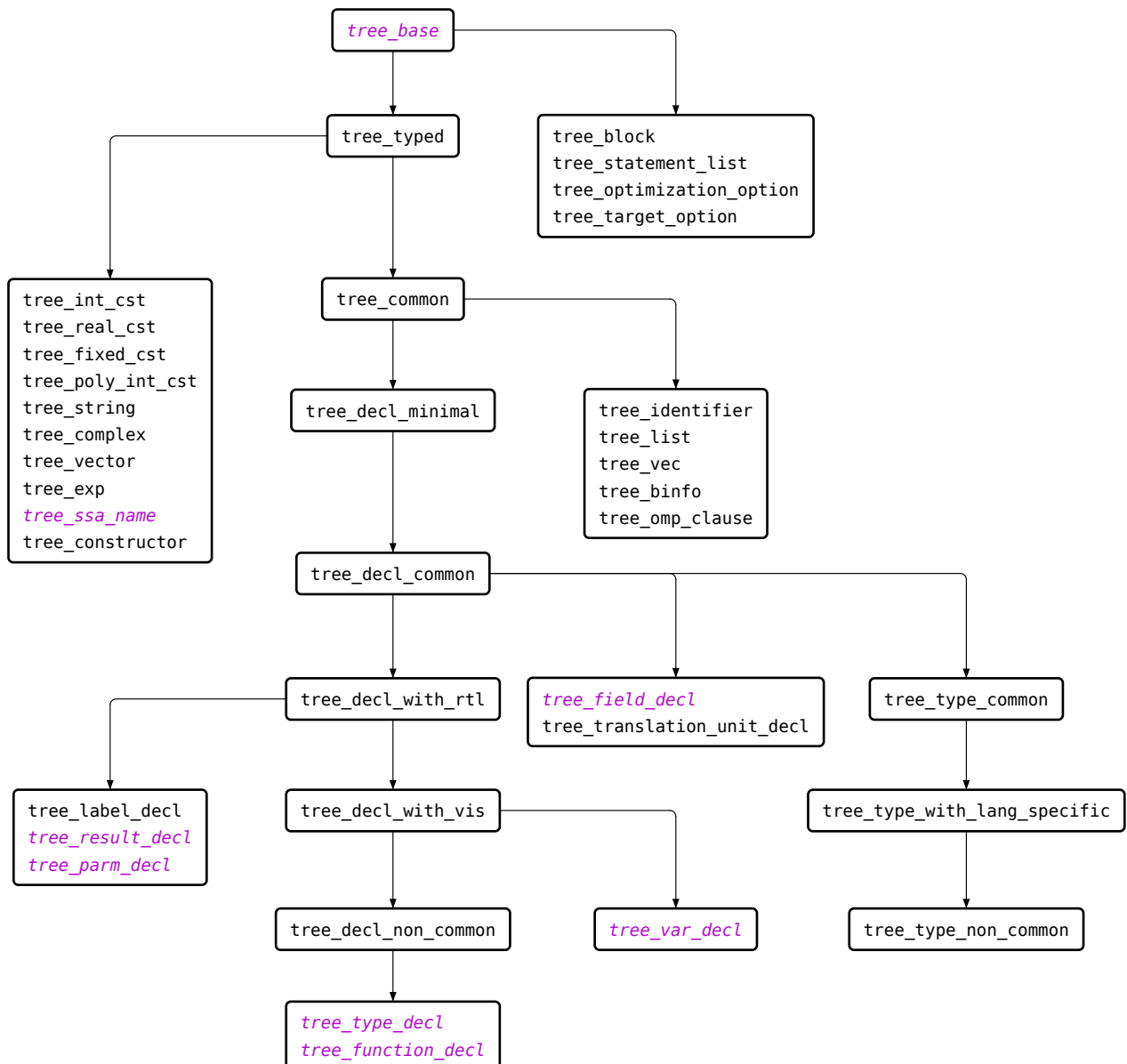
Figure 3: The structure hierarchy behind the tree_node union, starting from tree_base . The members of specific concern have been emphasized like this for clarity.
