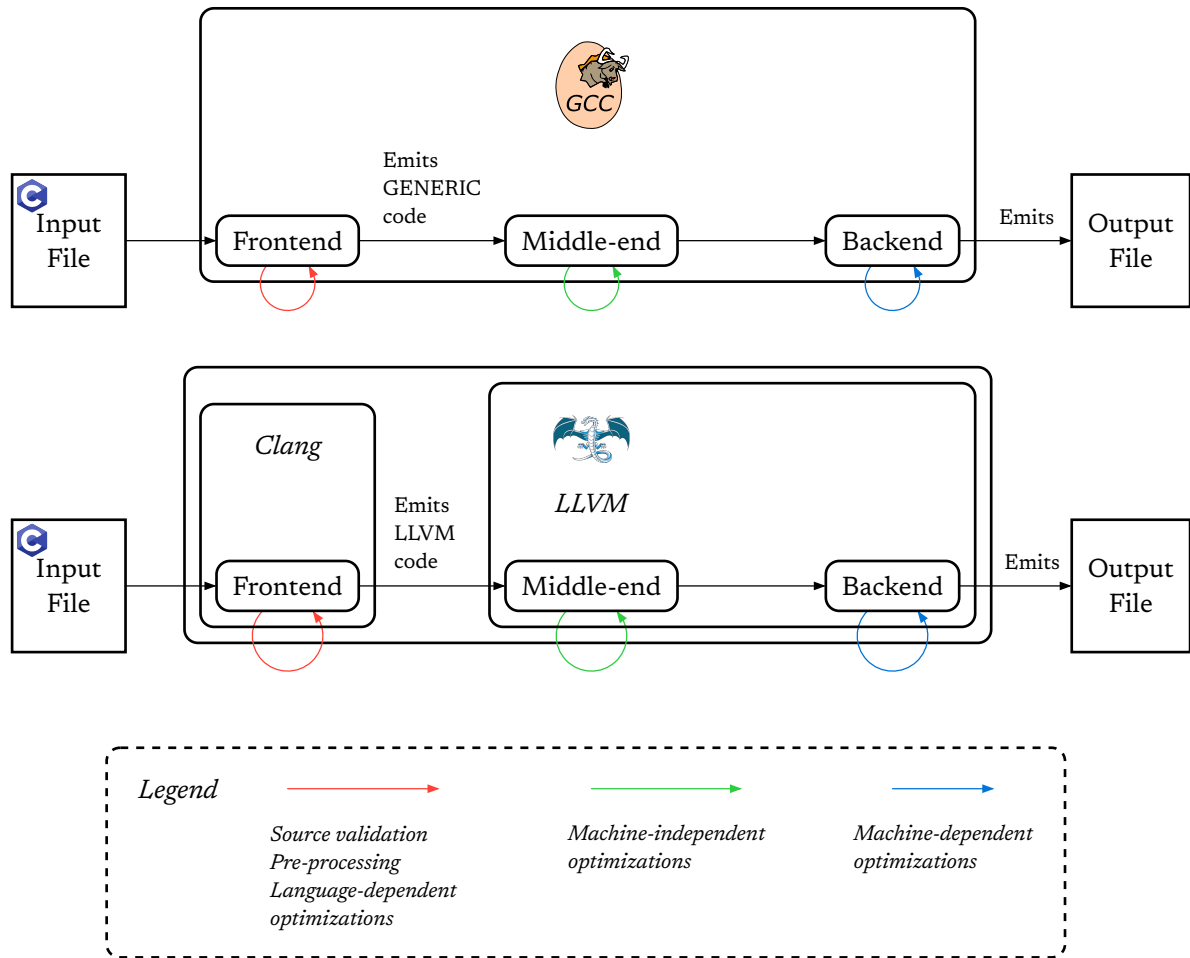
Figure 1: Compilation of a C file using GCC and Clang, from a black-box approach.
