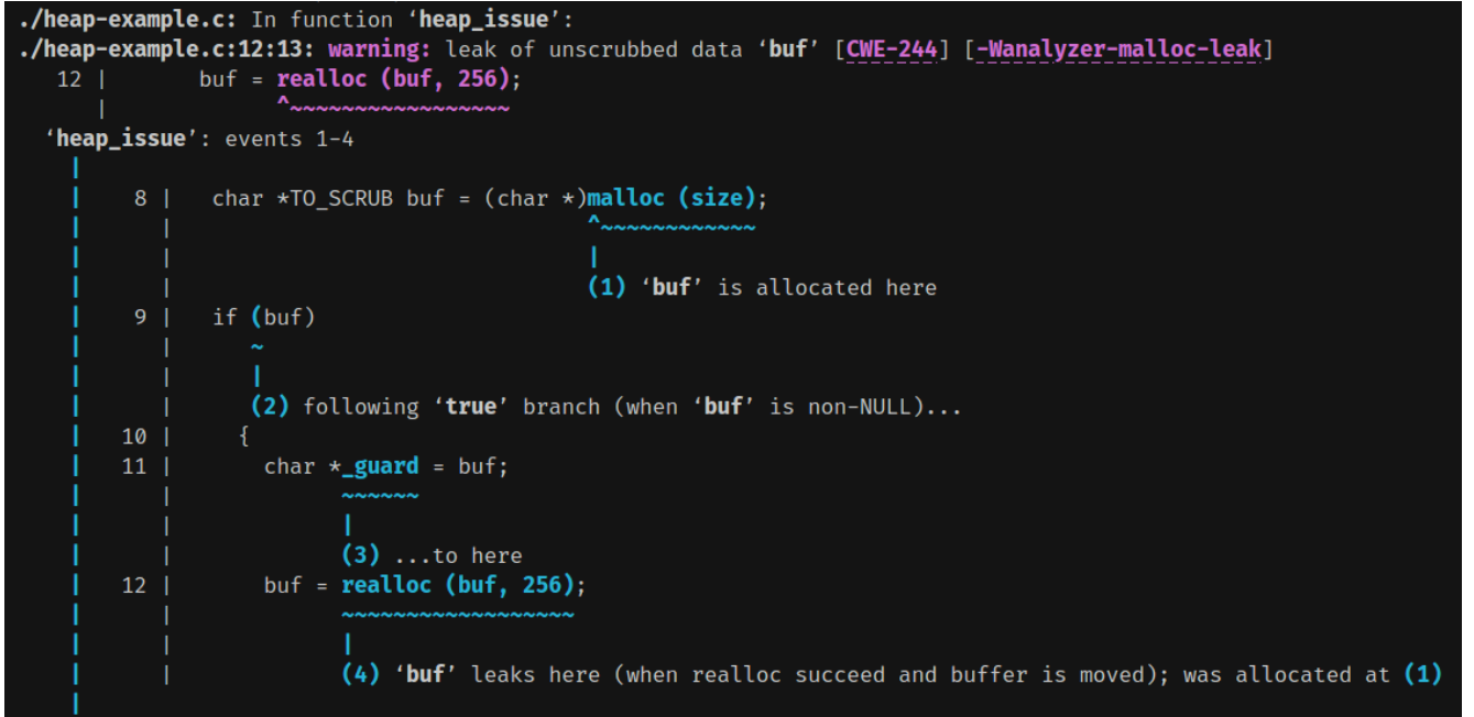
Image 2: GnuZero’s output when run over the heap example illustrated in Listing 16.
