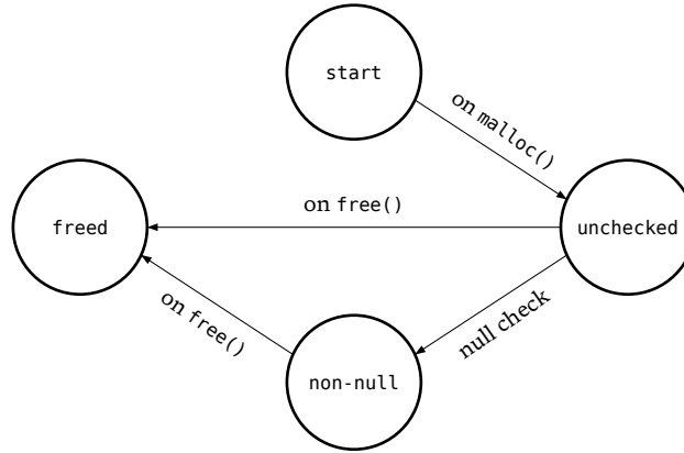
Figure 18: Simplified malloc state machine representation. For clarity, some transition edges have been removed, such as calls to realloc , alloca , or C++’s new operator.
