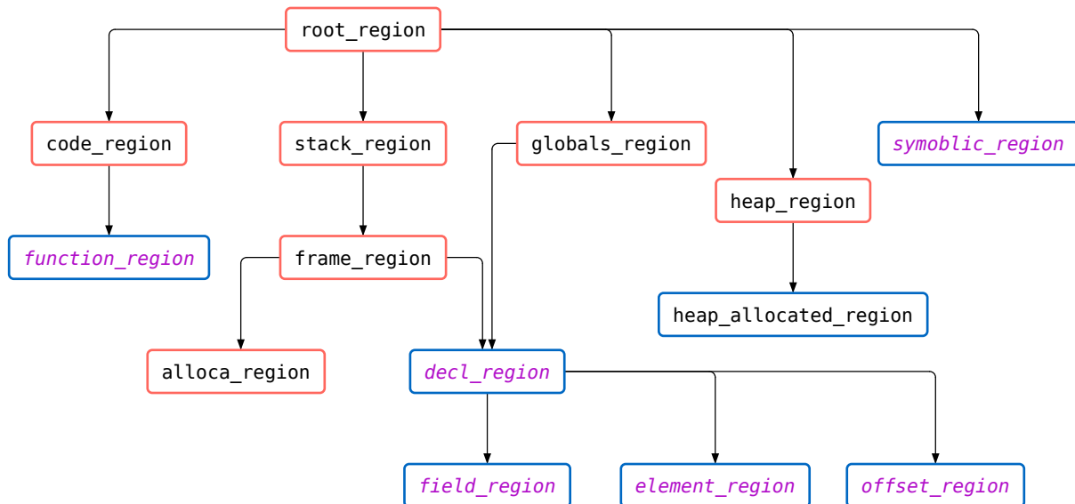
Figure 15: A Directed Acyclic Graph (DAG) representing the parenting relationship between the different regions implemented by the GSA, with typed region highlighted as those are the primary regions used during an analysis. The red nodes represent space region and the blue ones represent concretes region.
