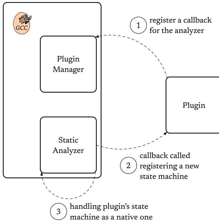
Figure 19: GCC/GSA plugin's registration workflow.
