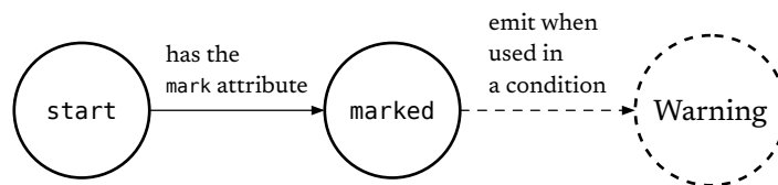
Figure 20: A dummy state machine emitting a warning when a variable with the mark attribute is used in a condition.
