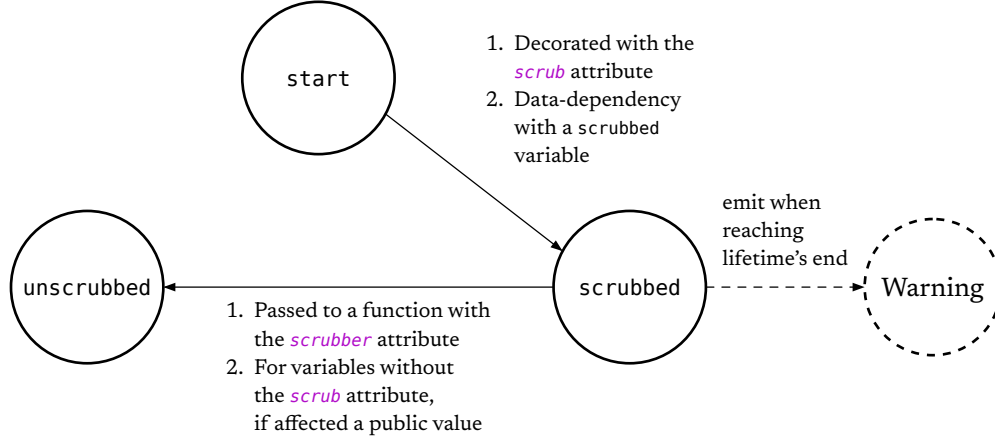
Figure 24: The zeroization state machine as implemented in GnuZero.
