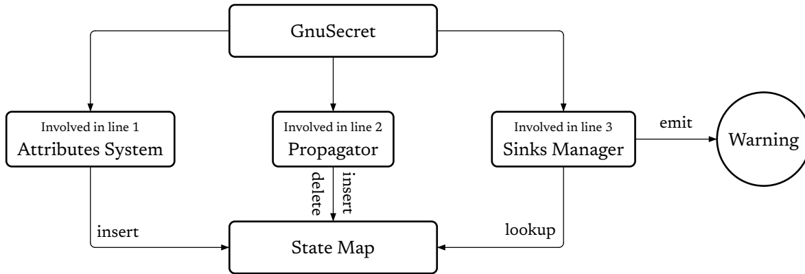
Subfigure 25.2 GnuSecret Components Architecture.
