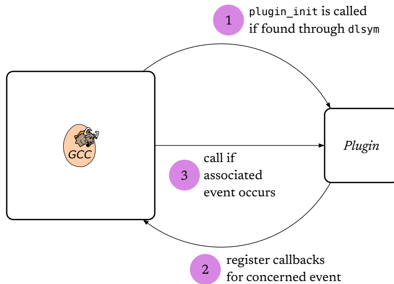
Figure 11: Relation between a plugin and GCC when invoked on Command Line Interface (CLI) with -fplugin=/path/to/plugin.so .
